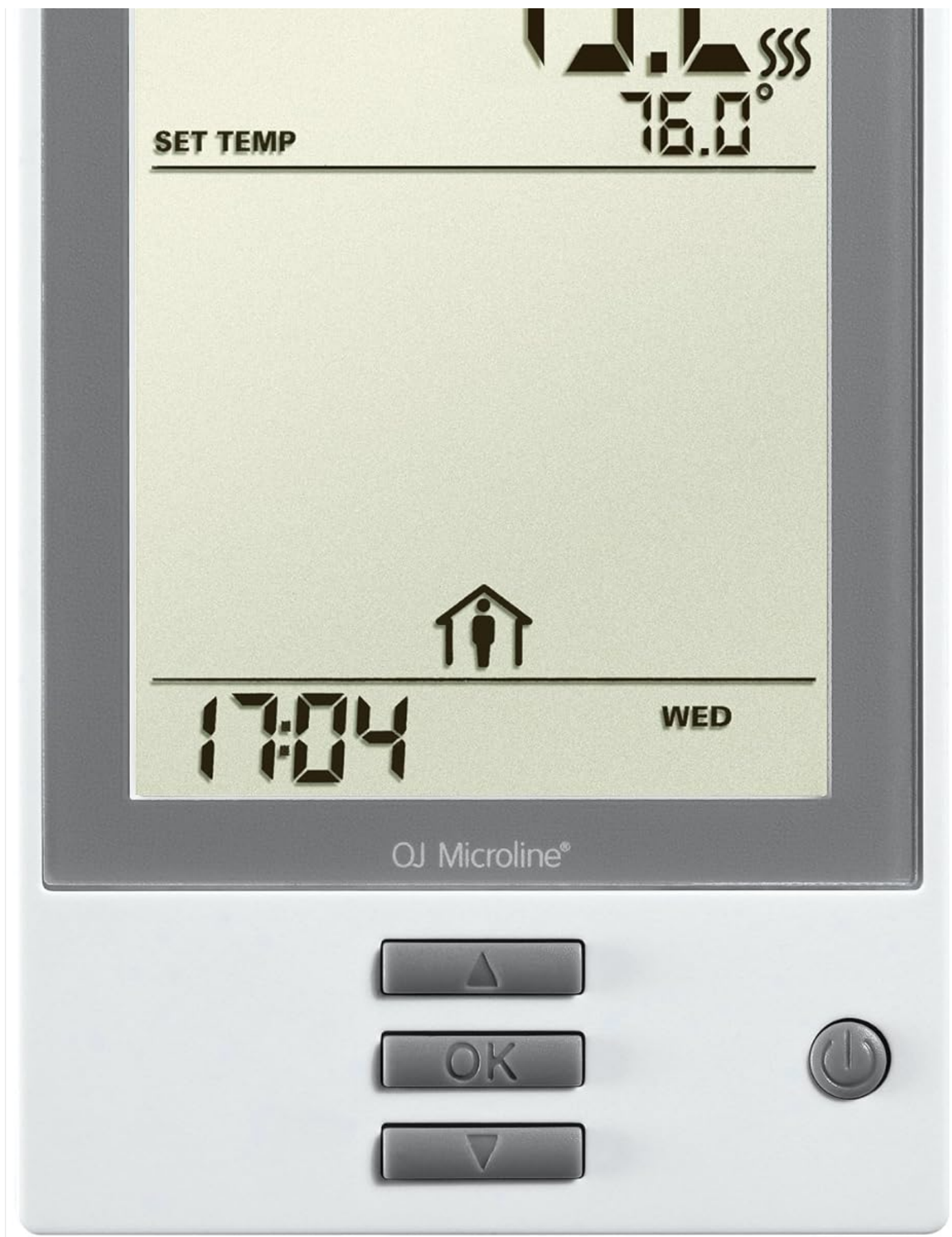
Figure 1: Front view of the WarmlyYours nHance Programmable Thermostat, showing the large digital display and control buttons.
