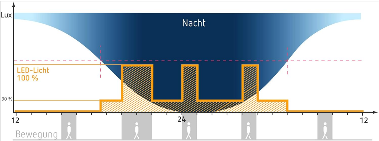
Figure 3: Operational diagram showing light activation (LED-Licht 100%) based on ambient light (Lux) and detected movement (Bewegung) over a 24-hour cycle (Nacht indicates night).
