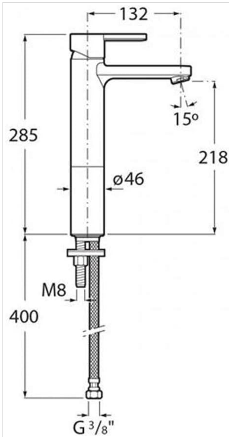
Image 2: Technical diagram showing the dimensions of the Roca NAIA MEZ LAV ALTO LISO tap and its installation components, including the M8 bolt and G 3/8" flexible hoses.
