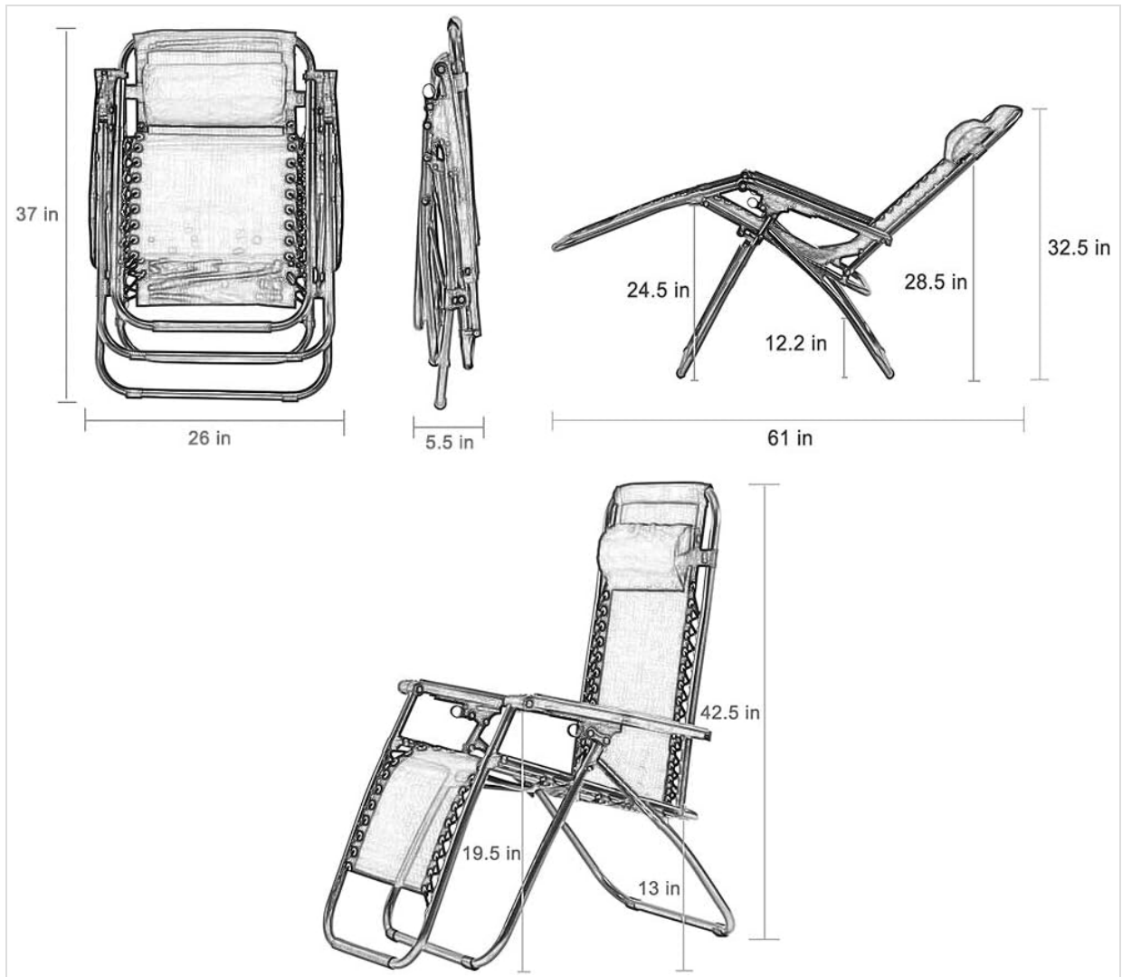
Figure 4: Folded dimensions of the FDW Zero Gravity Chair for storage.
