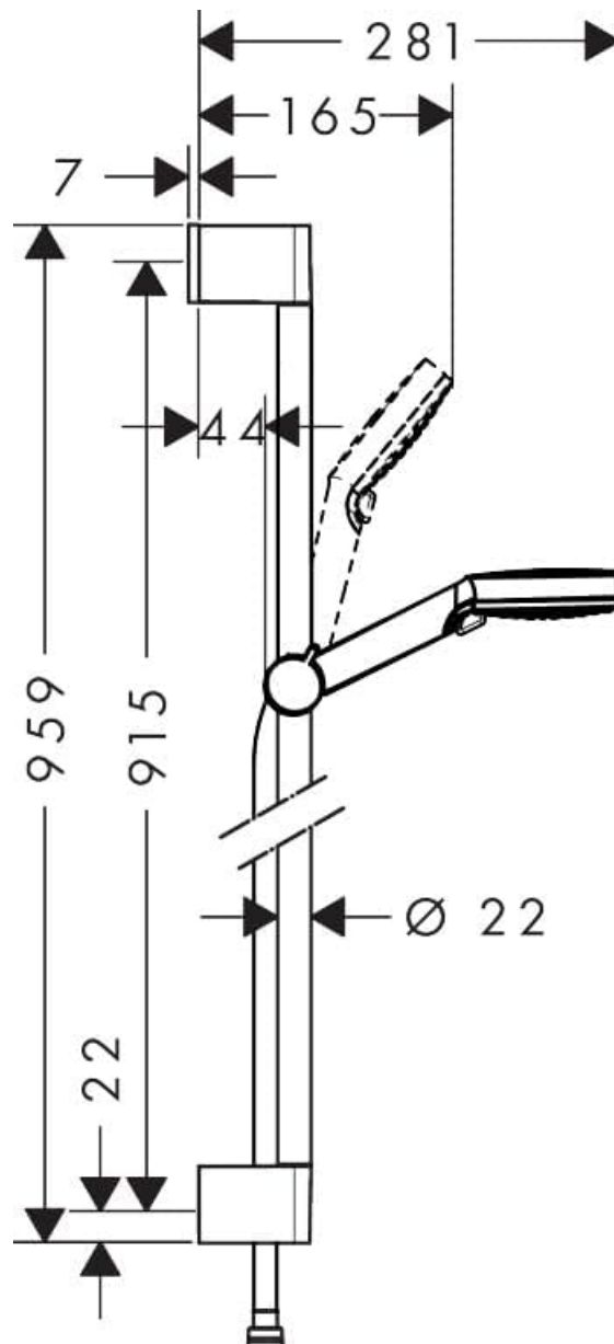
Image: Technical drawing illustrating the dimensions and mounting points for the shower rail.
