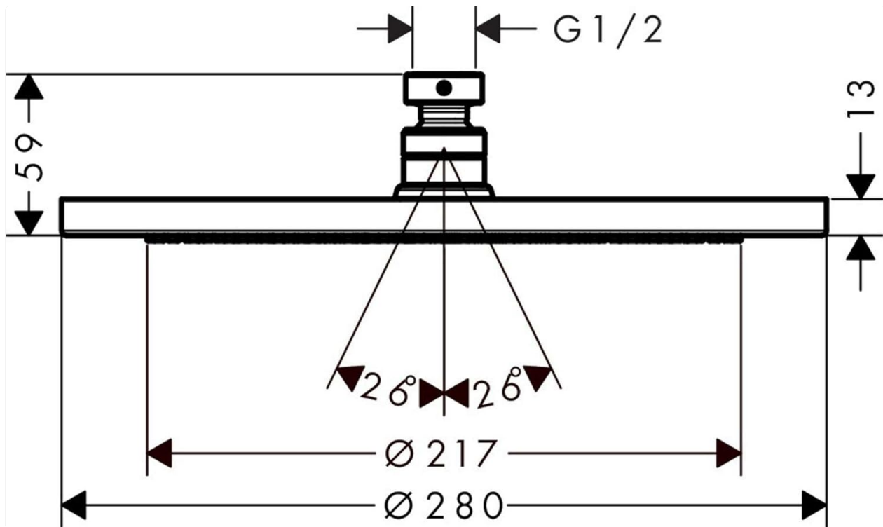
Technical drawing showing the dimensions of the hansgrohe Cromo 280 Air Overhead Shower, including the 280mm diameter and G 1/2 connection.
