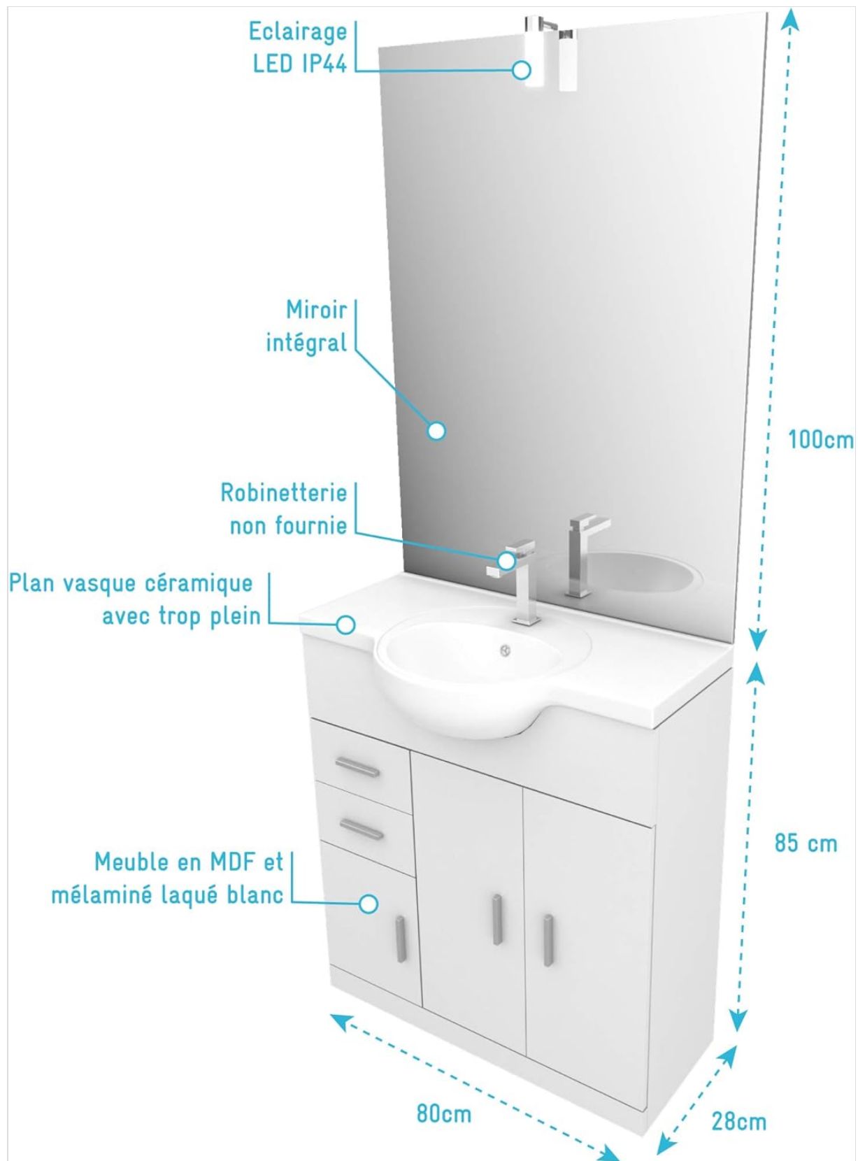
Image 4: Dimensional diagram of the Aurlane LAV301 Bathroom Vanity Unit. This diagram illustrates the key measurements of the unit, including the cabinet width (80cm), depth (28cm), cabinet height (85cm), and total mirror height (100cm).
