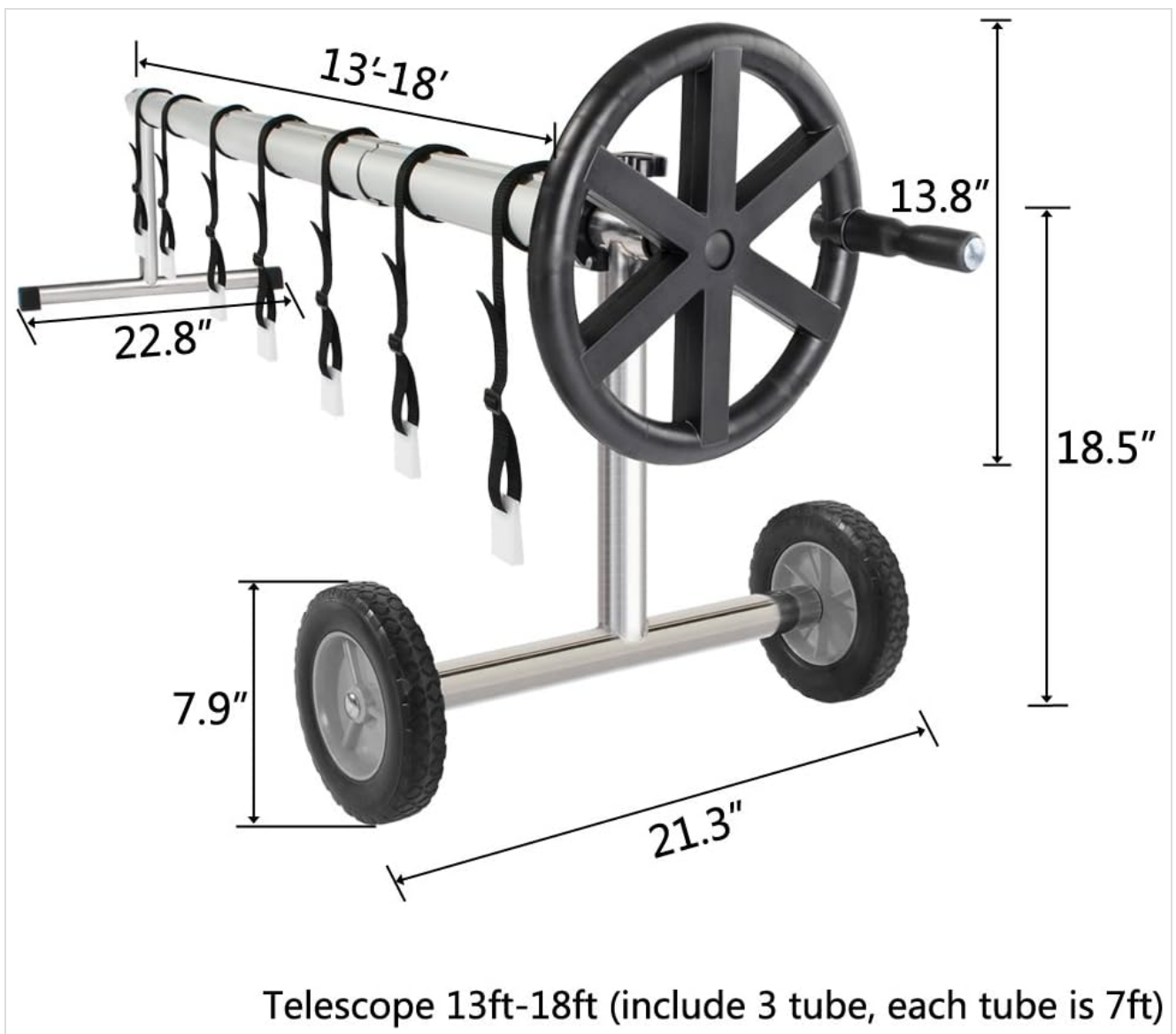
Figure 2: Product Dimensions and Adjustable Width.
