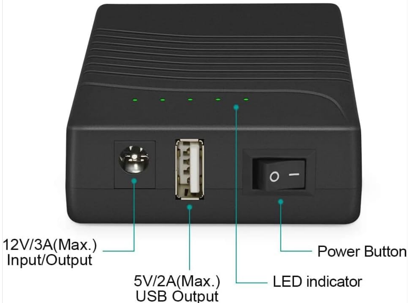
Figure 3.1: Front panel of the battery pack with labeled ports.
