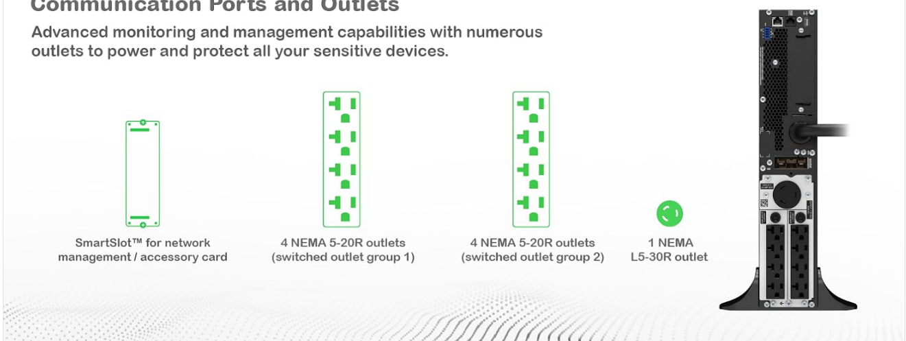
Figure 3.3: Rear panel view detailing the communication ports and power outlets, including SmartSlot, NEMA 5-20R, and NEMA L5-30R connections.
