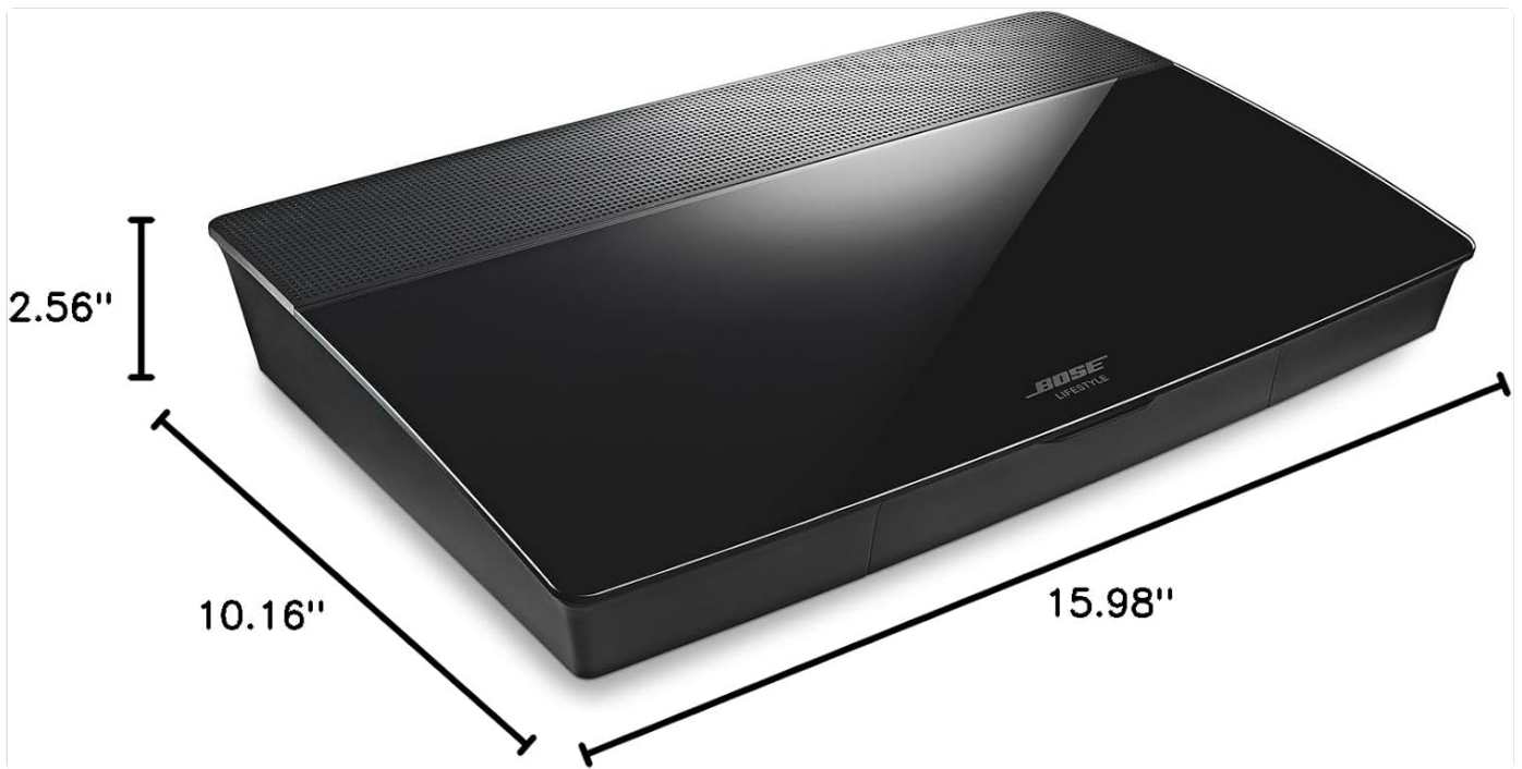
Figure 8: Console dimensions.
