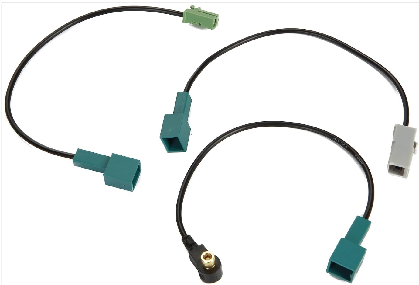
Image: The Maestro Acc-SAT-TO2 adapter kit, showing the various connectors for satellite radio and GPS antennas.
