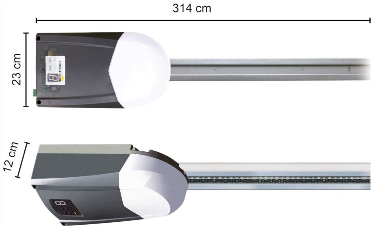
Figure 4.1: Dimensions of the Smart Drive garage door opener unit and rail.
