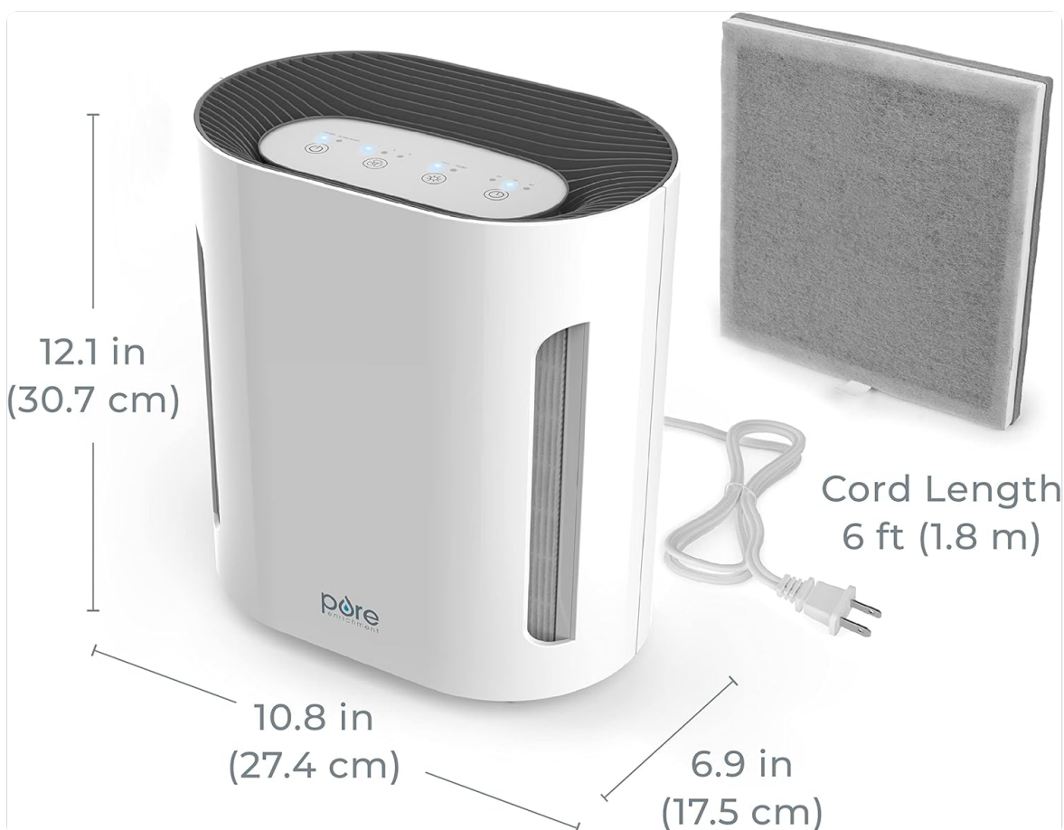
Image: Visual representation of the PureZone Air Purifier's dimensions.
