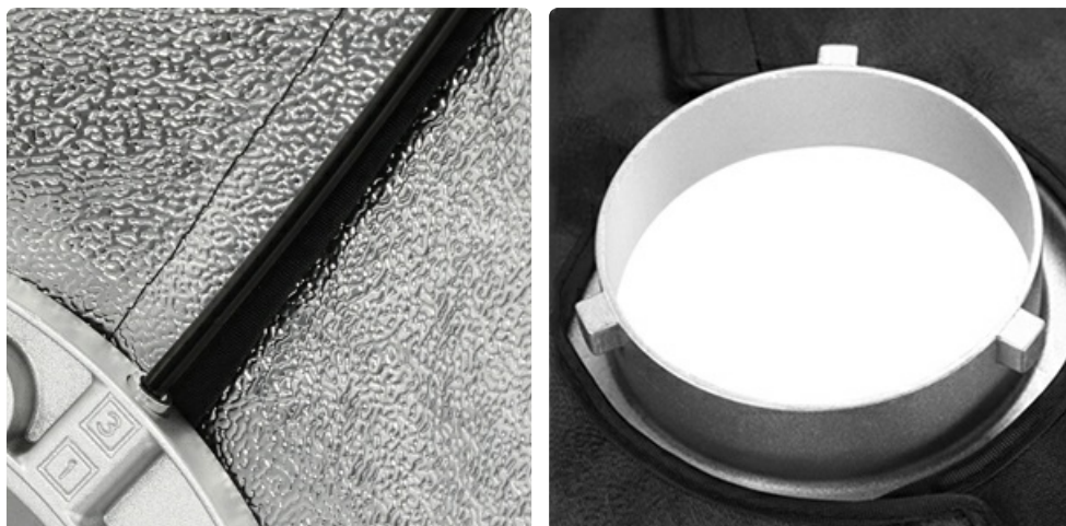
Image 3.1: Inserting a support rod into the speedring (left) and detail of rod ends (right).
