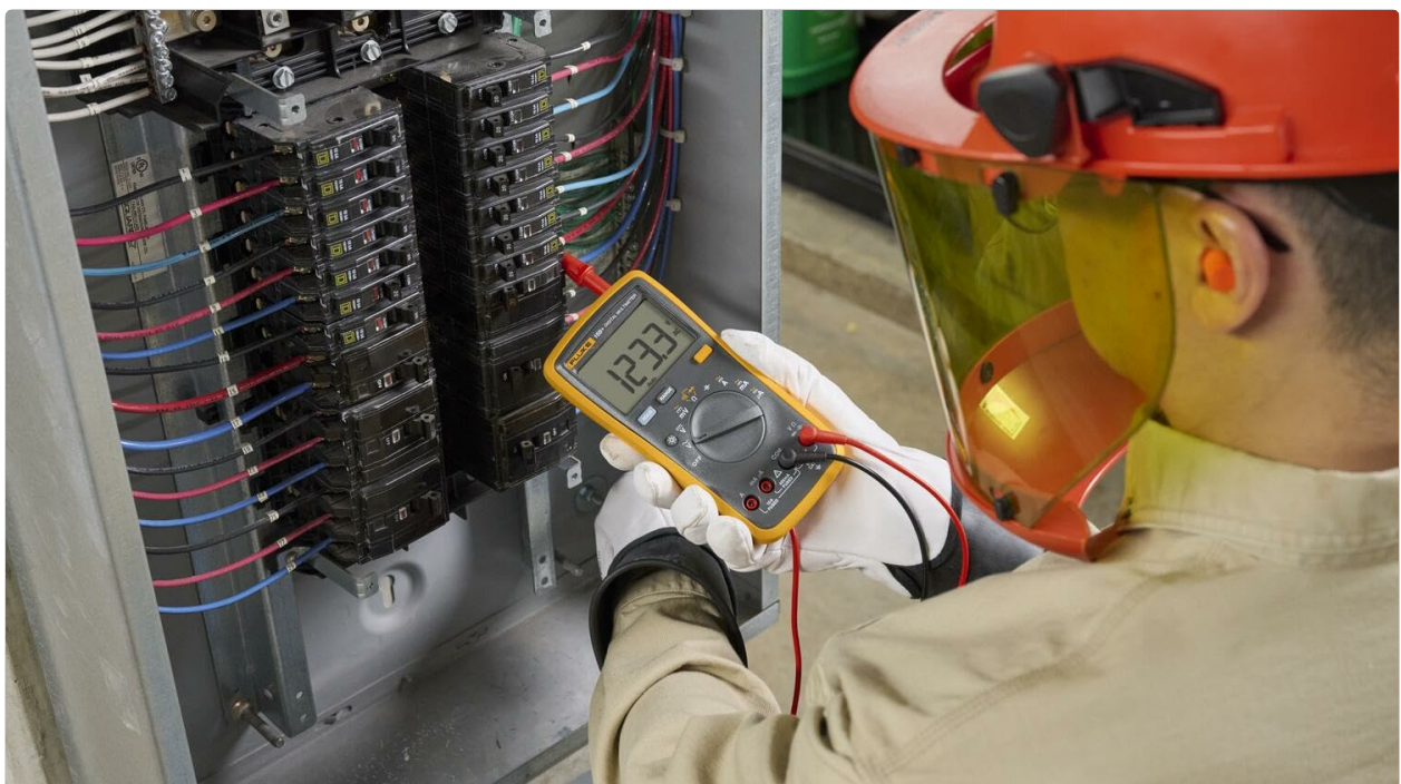
Image: A technician wearing safety gear, using the Fluke 15B+ Digital Multimeter to take a reading inside an electrical panel.
