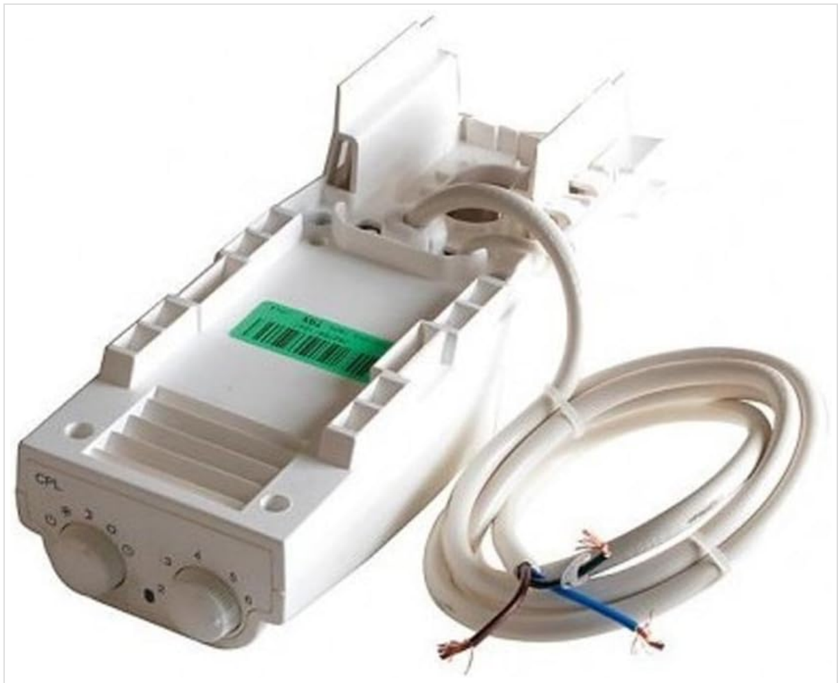
Figure 1: Acova Tax-Tag Thermostat Control Unit, Model 895010. This image shows the white plastic control unit with two rotary knobs on the front, labeled 'CPL' and with numerical markings. A green sticker with a barcode is visible on the top surface. Electrical wiring, including a white coiled cable with exposed brown and blue wires, is connected to the unit, indicating its electrical nature.
