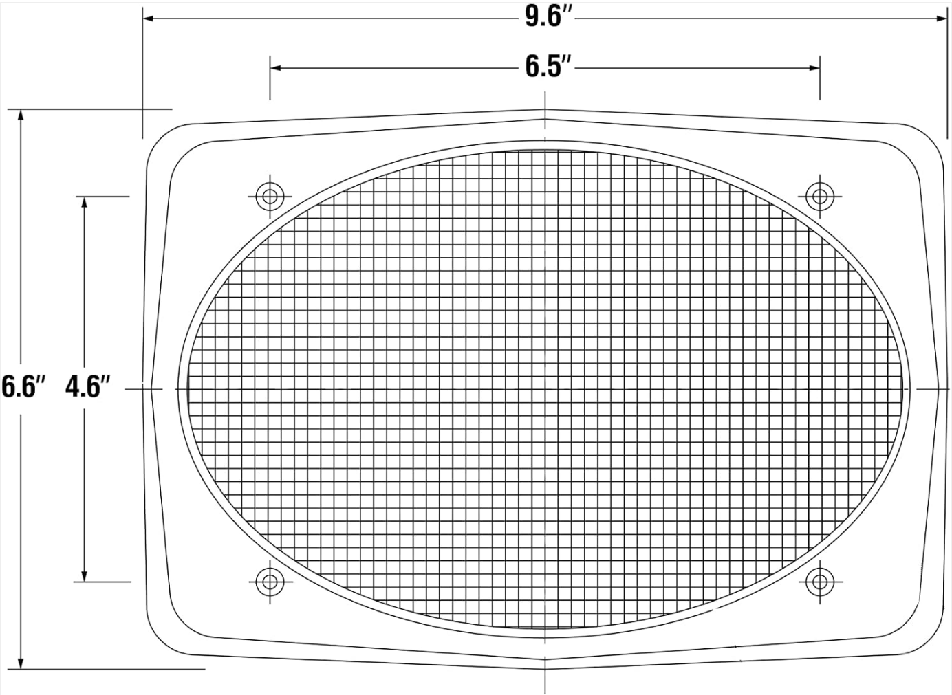
Image: Technical drawing showing the dimensions of the 6x9 speaker grill, including overall length, width, and mesh area.
