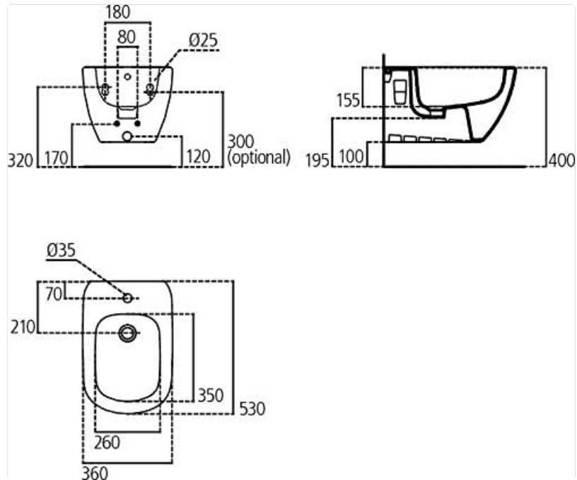
Figure 2: Technical drawing illustrating the dimensions and connection points for the Ideal Standard T355201 Suspended Tesi Bidet. Refer to these measurements for accurate installation planning.
