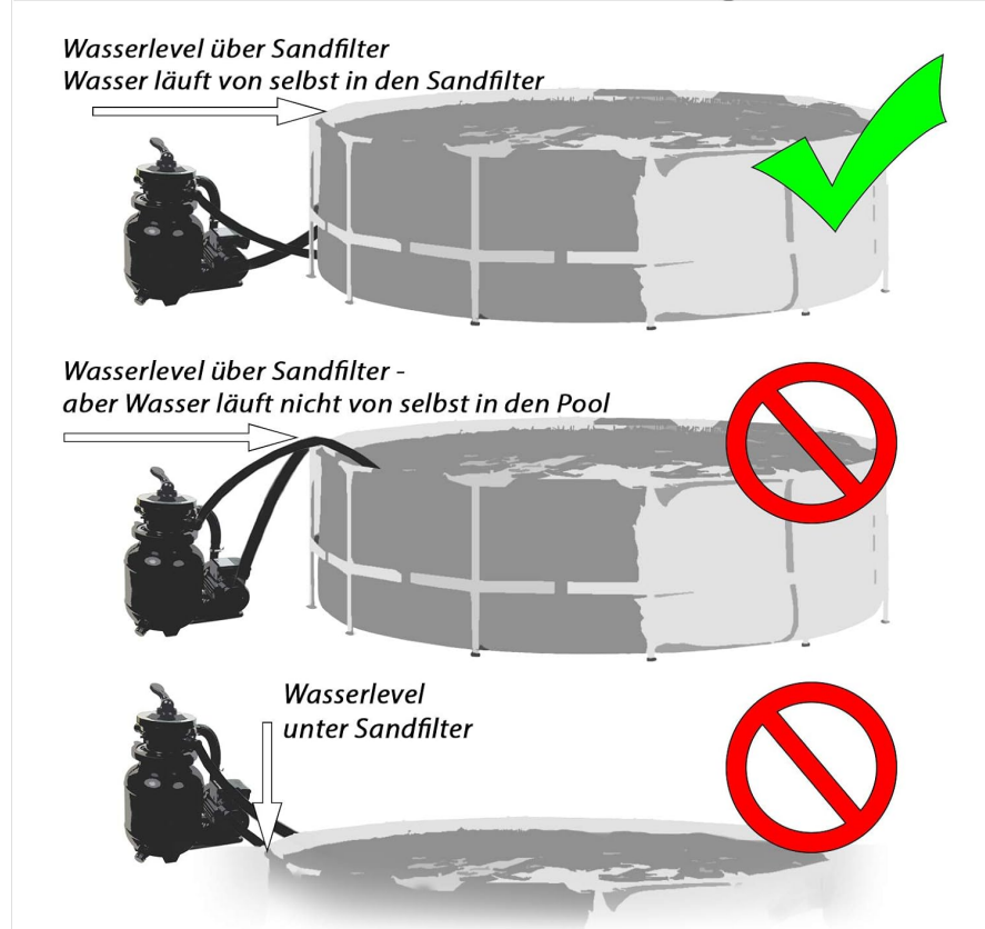
Figure 5: Illustration of correct (top) and incorrect (middle, bottom) placement of the sand filter relative to the pool's water level for optimal gravity flow.
