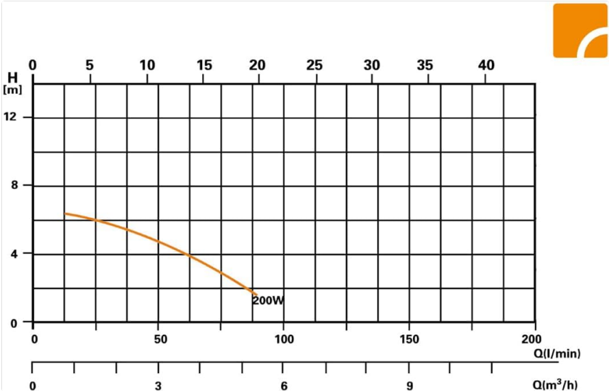
Figure 6: Pump performance curve, illustrating flow rate (Q) versus head (H) for the 200W pump.
