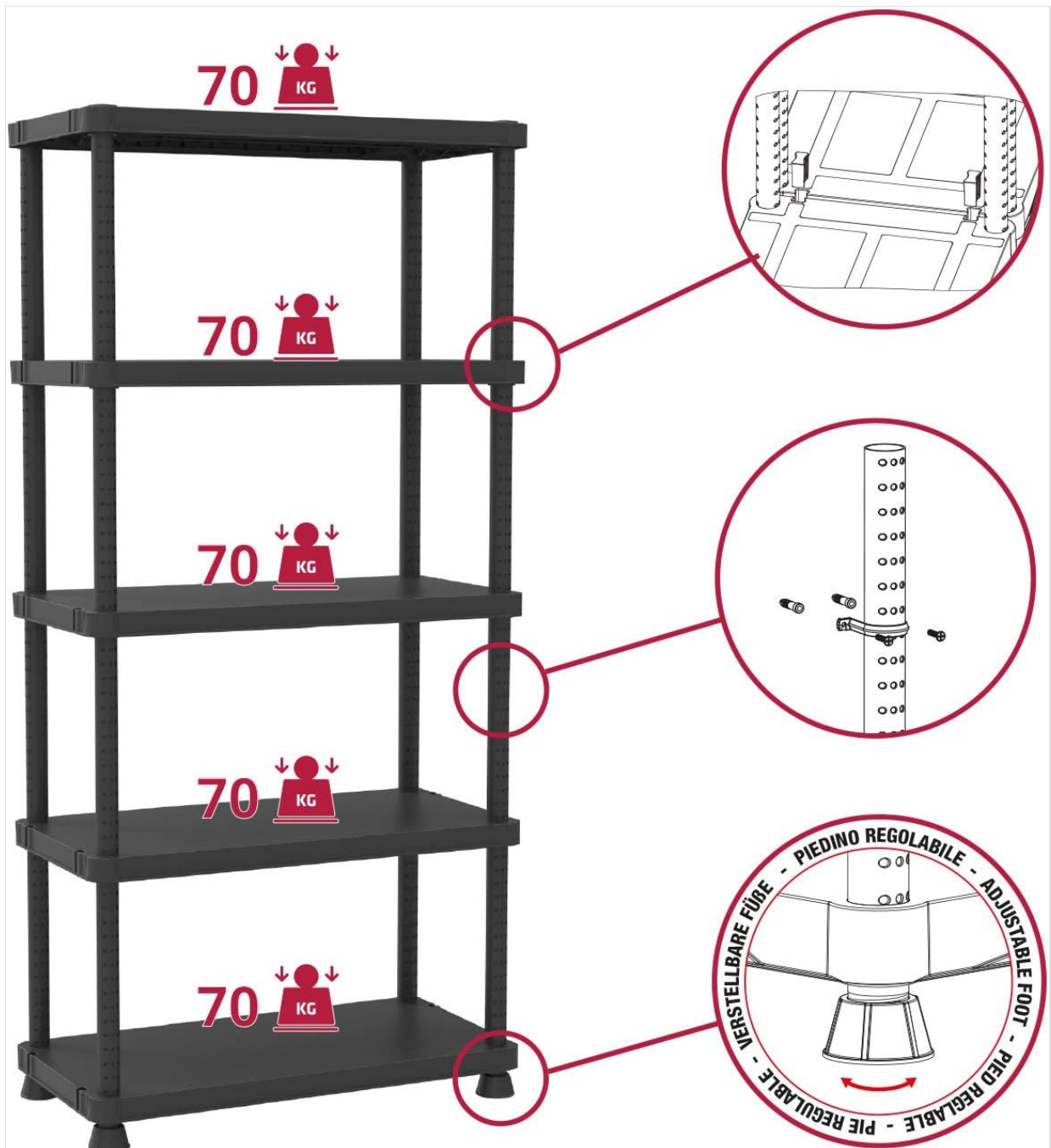
Figure 3: Detail of adjustable feet and post connections.
