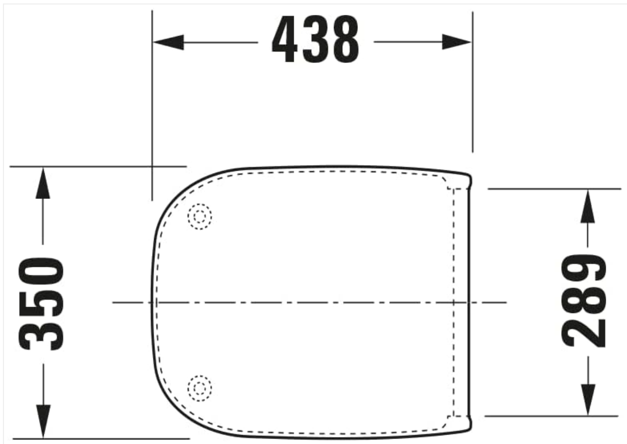
Image 4.1: Dimensional drawing of the Duravit D-Code Compact toilet seat (measurements in mm).
