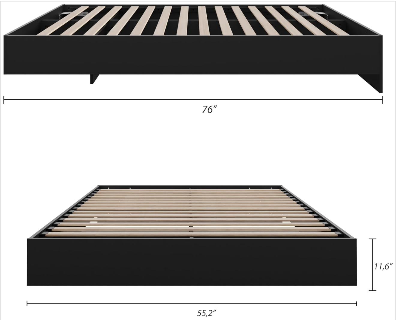
Figure 7.1: Dimensional diagram of the Nexera Full Platform Bed.
