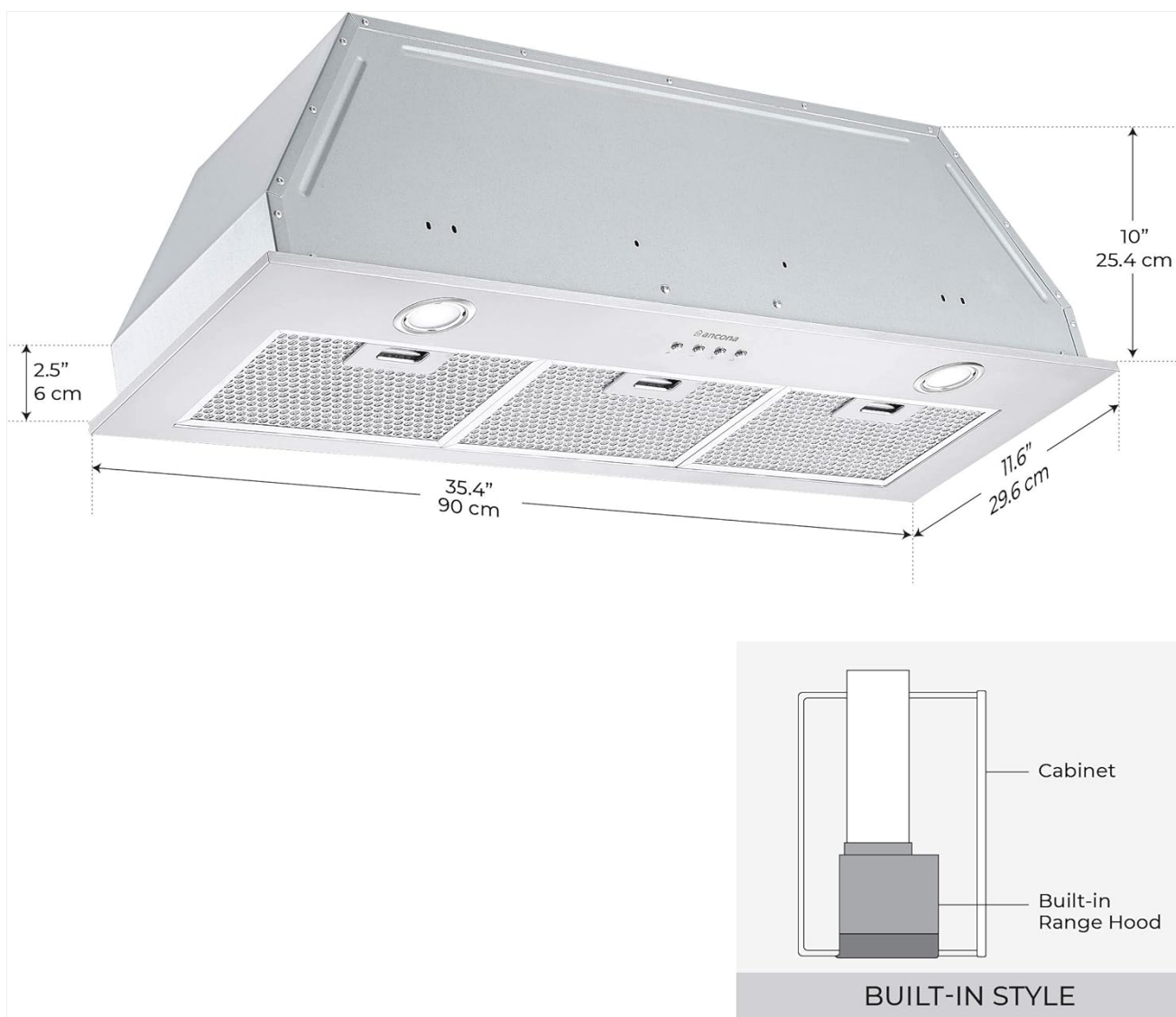
Image 4.1: Detailed dimensions of the range hood and a schematic illustrating its built-in installation within a cabinet.
