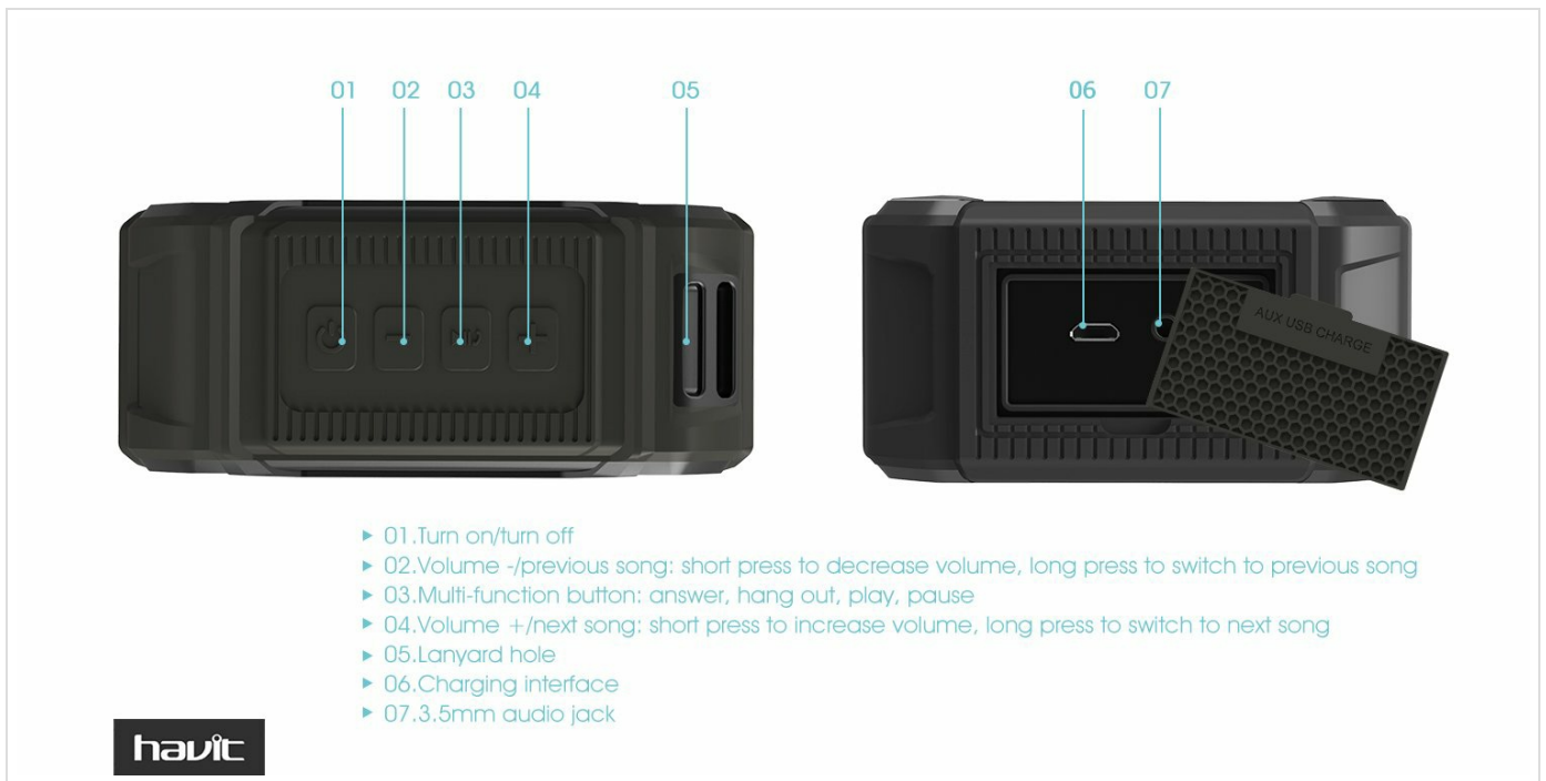
Figure 6: Button layout and functions of the HAVIT HV-SK533BT speaker.
