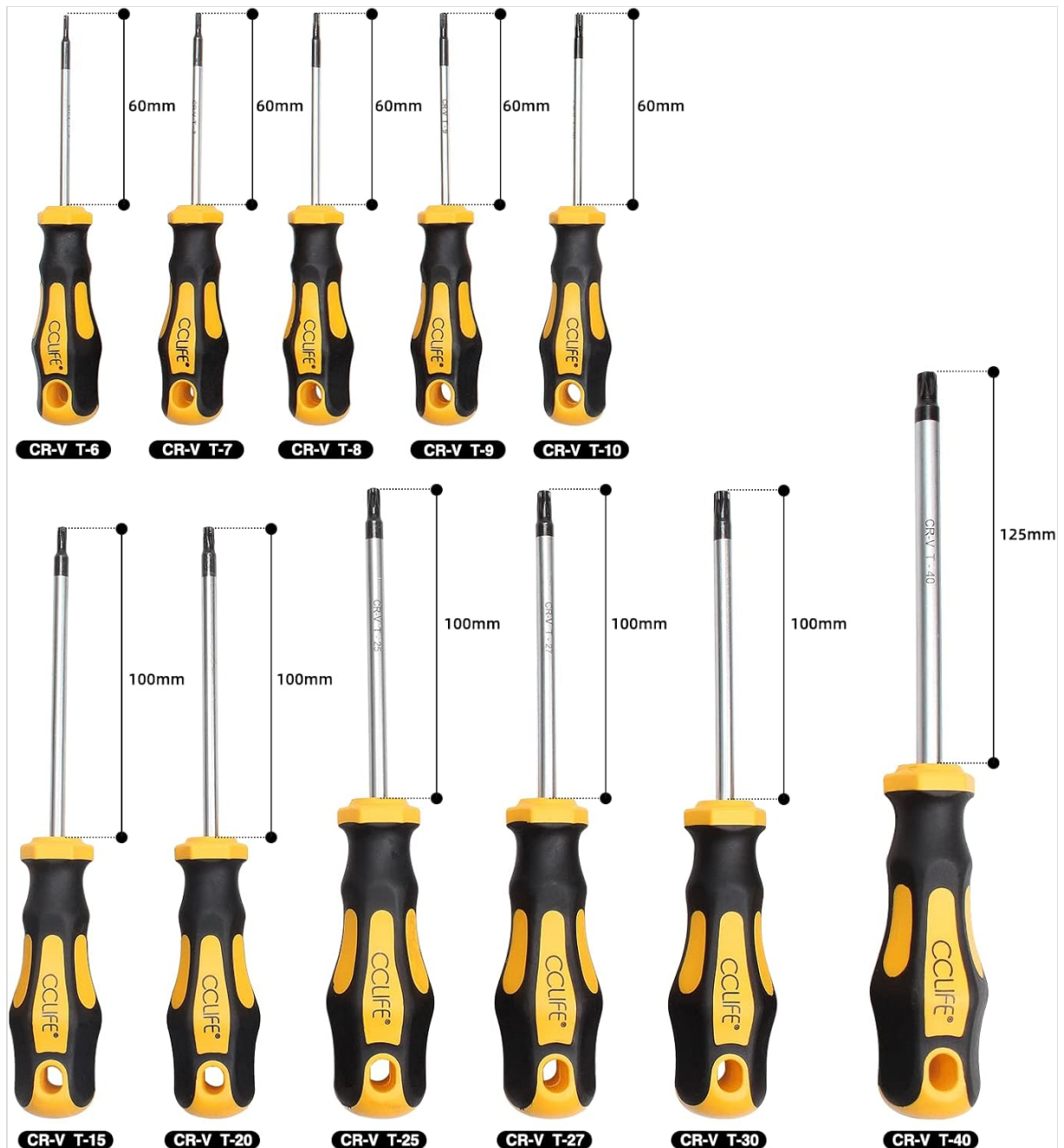
Image 6.1: Dimensions of the CCLIFE Torx Screwdriver Set.
