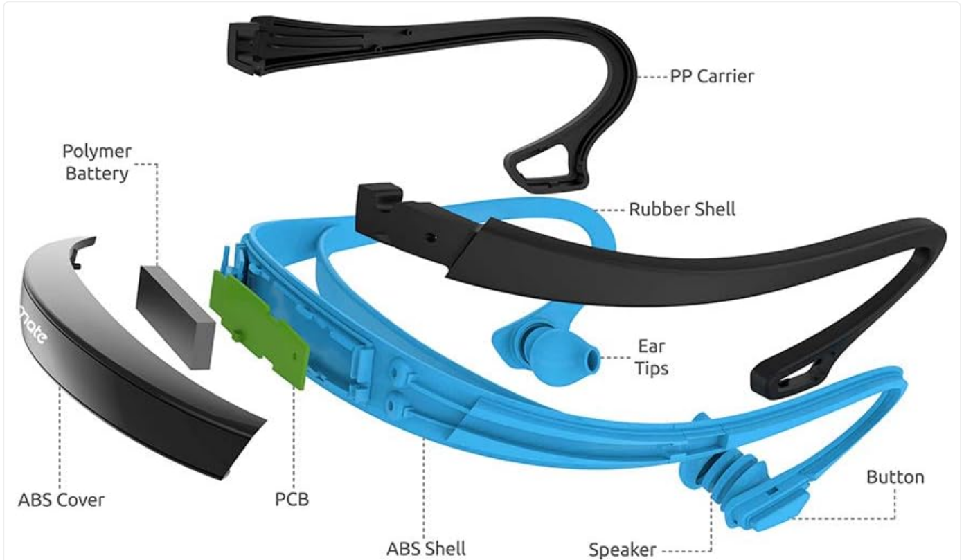
Figure 3: Exploded diagram showing the internal components of the Solix-1 headset, including the ABS cover, polymer battery, PCB, ABS shell, rubber shell, PP carrier, ear tips, and speaker.
