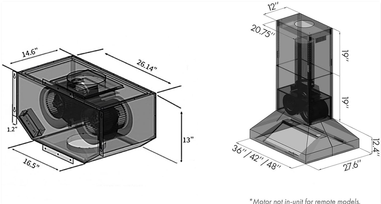
Dimensional drawing of the range hood and the remote blower unit.
