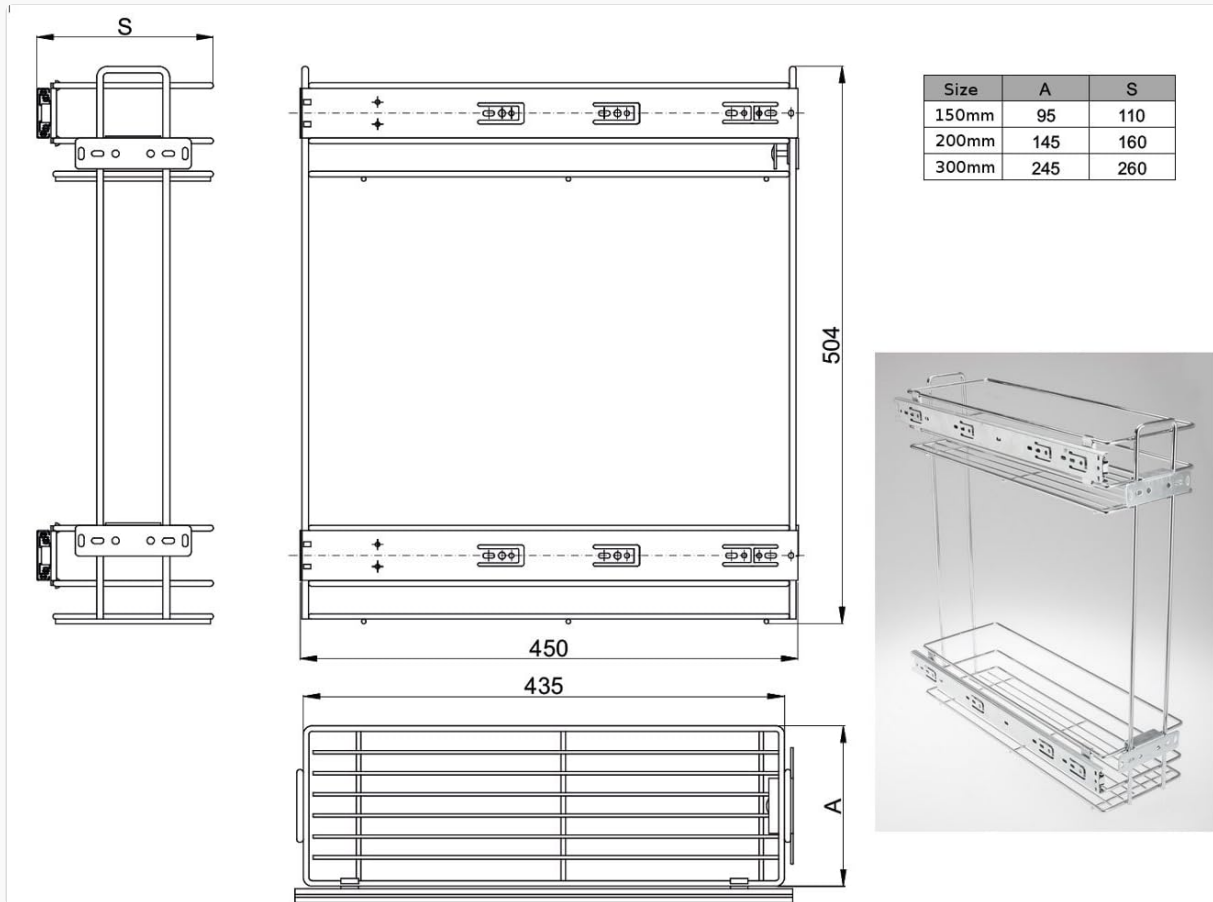
Figure 2: Technical Diagram with Dimensions for GTV Pull Out Wire Storage Basket
