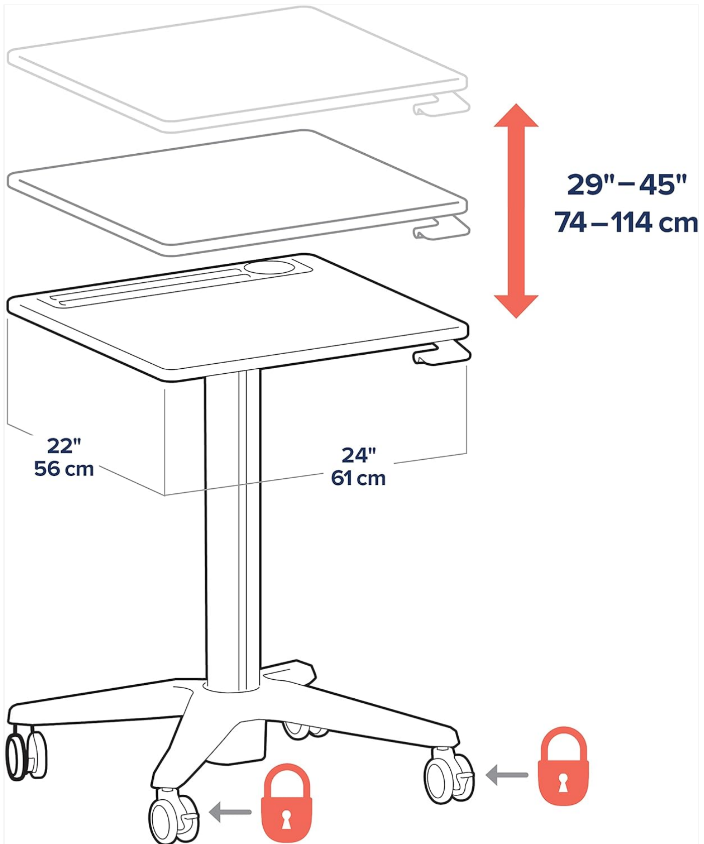
Figure 2: Assembly Diagram
