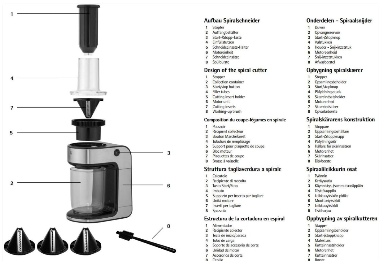
Figure 3.1: Exploded view of the spiral grater components.
