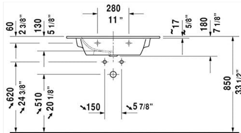
Image: Technical drawing illustrating the precise dimensions and installation requirements for the Duravit ME by Starck Sink. All measurements are critical for proper fit.
