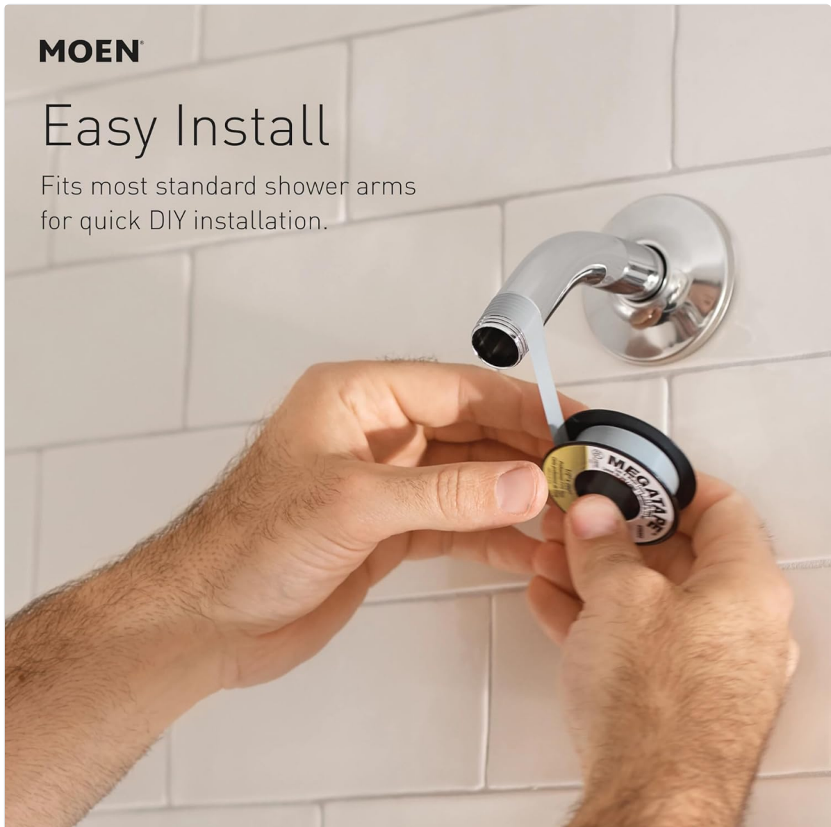
Image 2.1: Applying plumber's tape to the shower arm before installing the mounting bracket.
