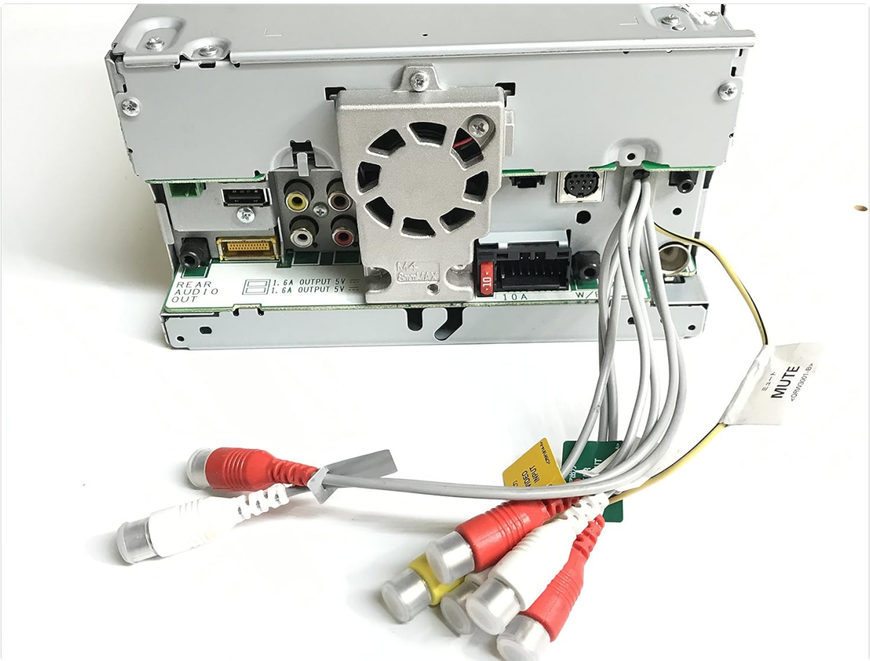
Figure 4.1: Rear connections of the AVIC-8200NEX with cables.
