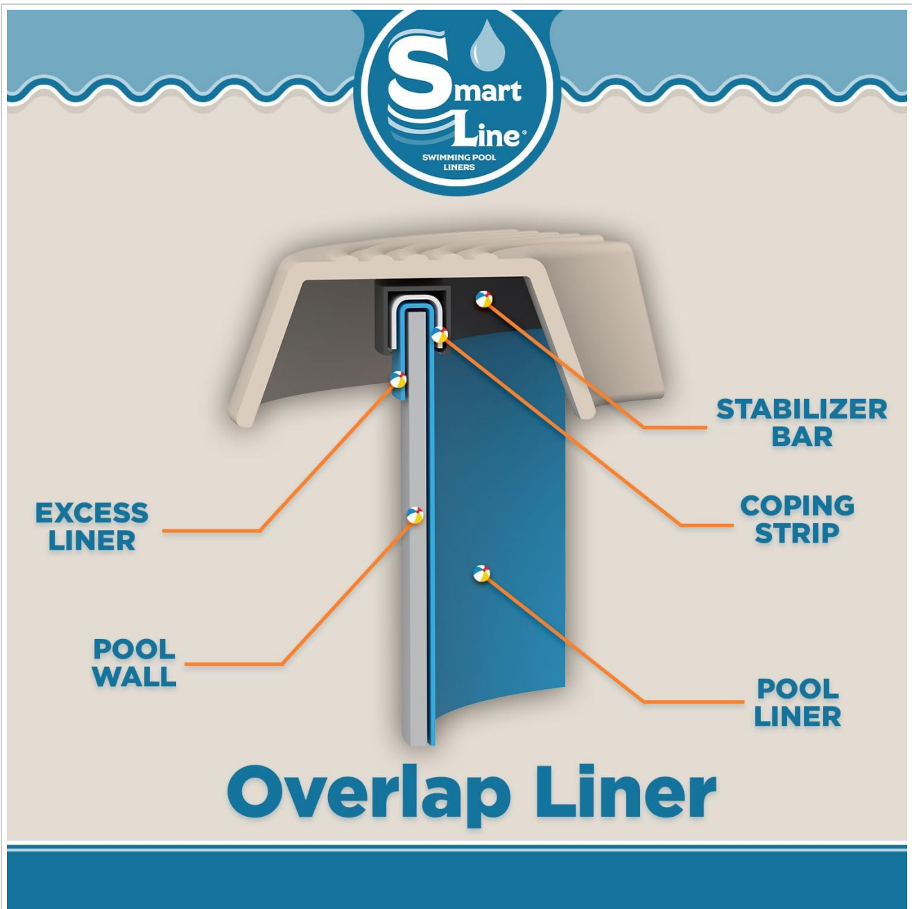
Figure 4: Diagram of an overlap liner installation, showing how the liner folds over the wall and is secured with coping strips.
