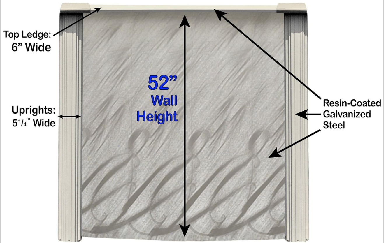
Figure 1: Key dimensions and material specifications of the Wilbar Meadows Reprieve 18 ft Round Above Ground Pool.
