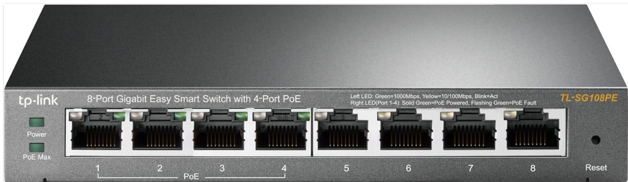
Figure 1: Front view of the TP-Link TL-SG108PE V3 8-Port Gigabit PoE Switch, showing 8 RJ45 ports, Power and PoE Max LEDs, and a Reset button. Ports 1-4 are marked for PoE.
