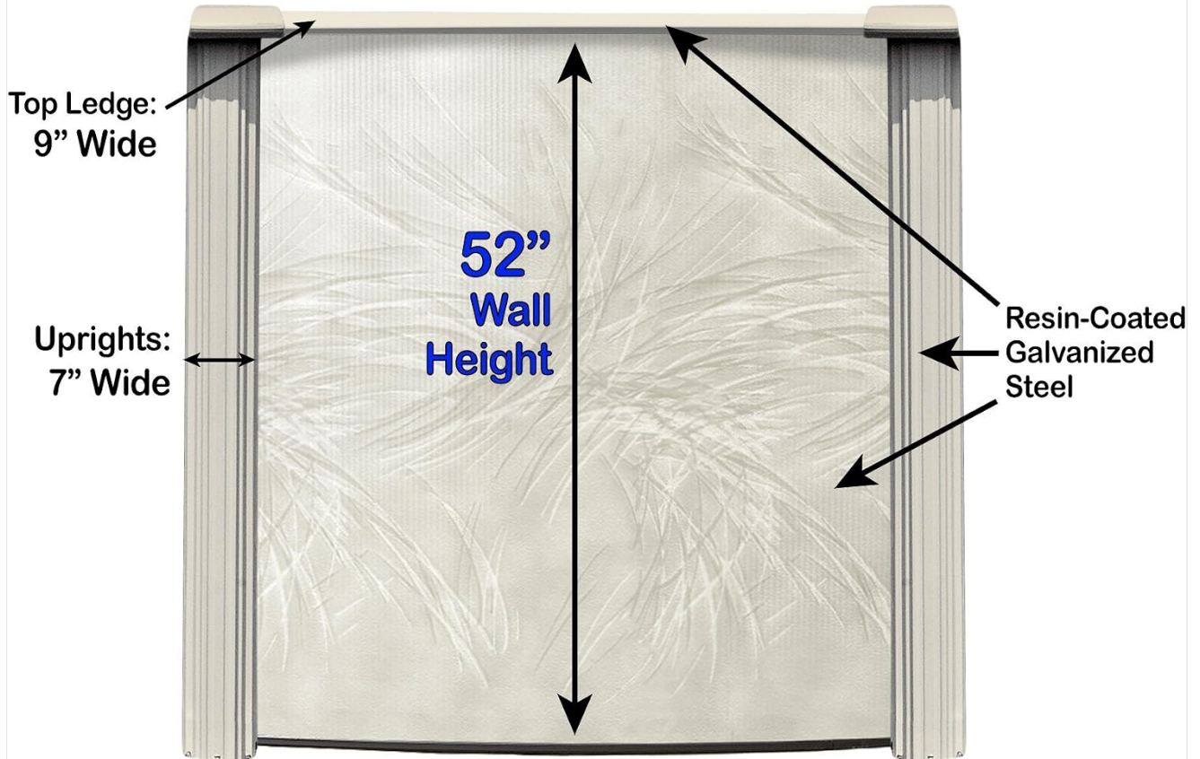
Image 2: A diagram illustrating the key dimensions of the 24 ft Round Fallston pool wall, including the 52-inch wall height, 9-inch wide top ledge, and 7-inch wide uprights. It also highlights the resin-coated galvanized steel construction.
