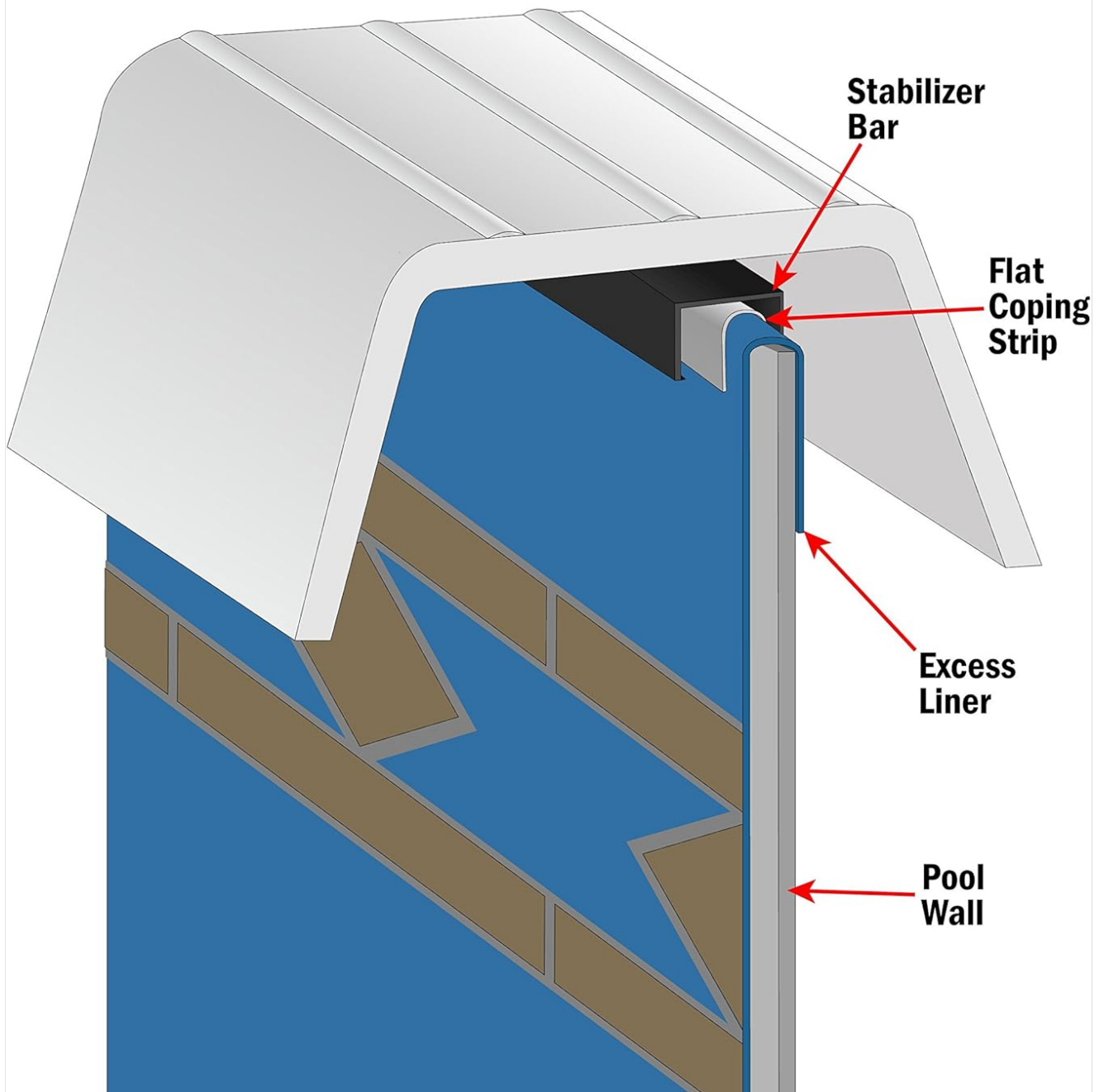
Image 4: A cross-section diagram illustrating how an overlap liner is installed, showing the excess liner folding over the pool wall and secured by a stabilizer bar and flat coping strip.
