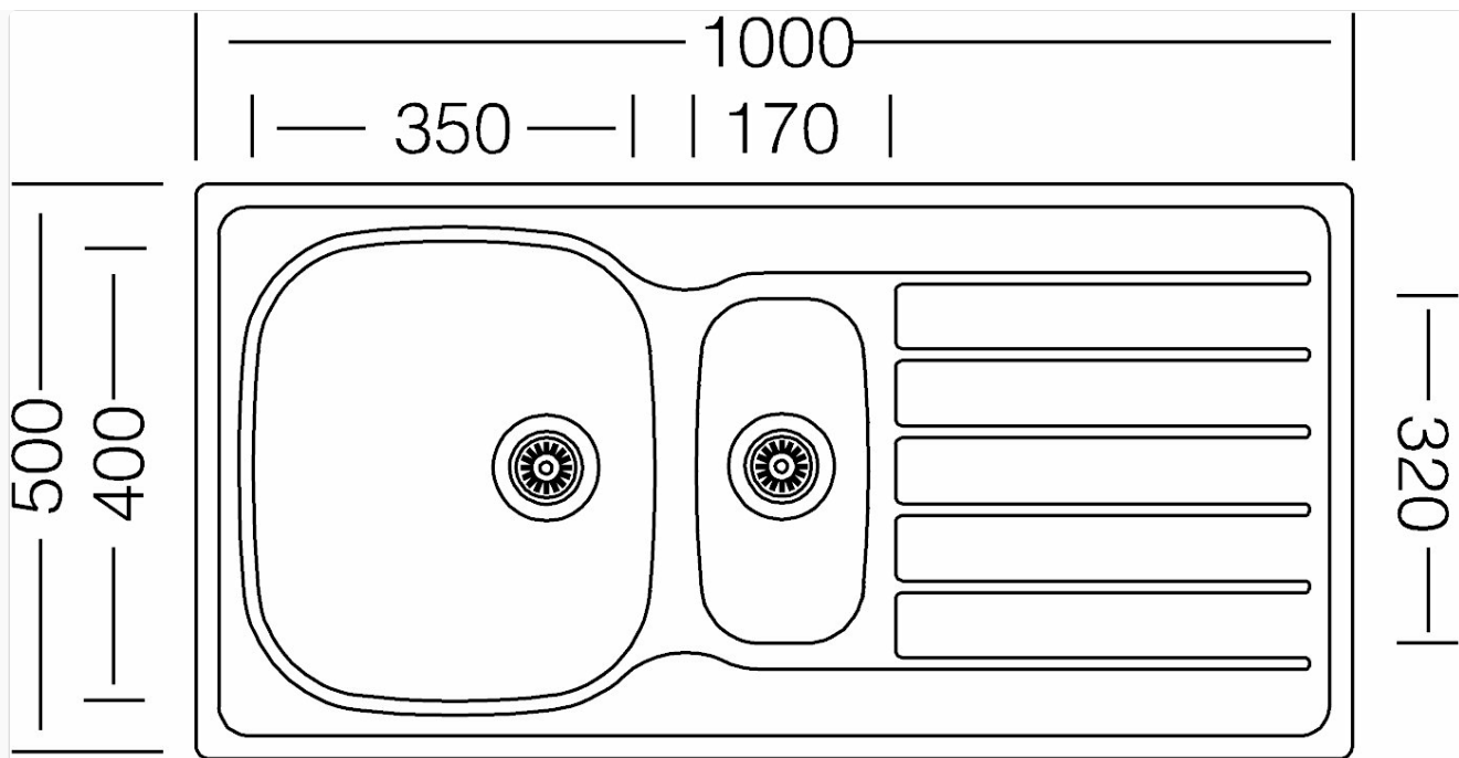
Figure 3.1: Detailed technical drawing showing the dimensions of the Respekta Dallas sink, including bowl sizes and overall length/width.
