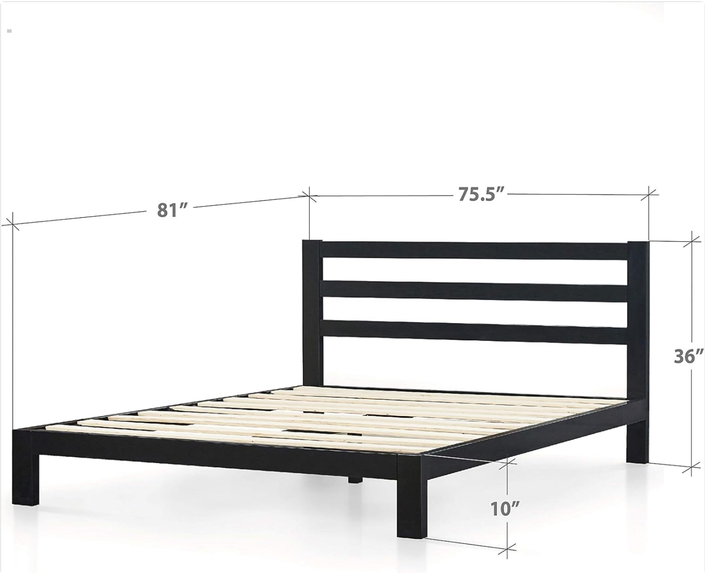
Figure 6: Detailed dimensions of the ZINUS Arnav Metal Platform Bed Frame.
