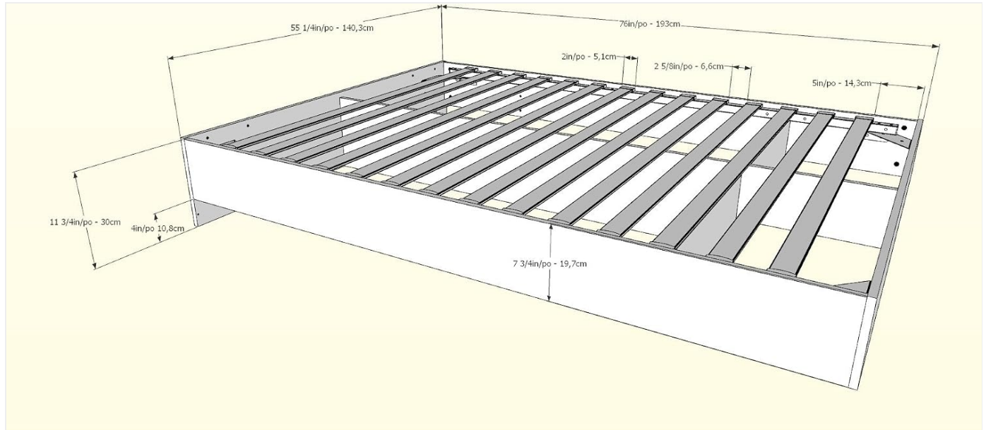
Image: Dimensional diagram of the Nexera Nocce Full Size Platform Bed, illustrating overall length (76 inches), width (55.25 inches), and height (11.75 inches), along with internal support structure measurements.
