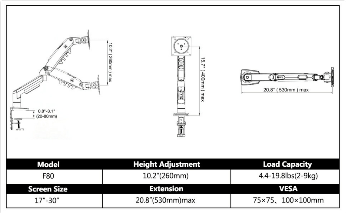
Image: Technical drawing showing the dimensions, screen size compatibility, and load capacity of the F80 monitor mount.
