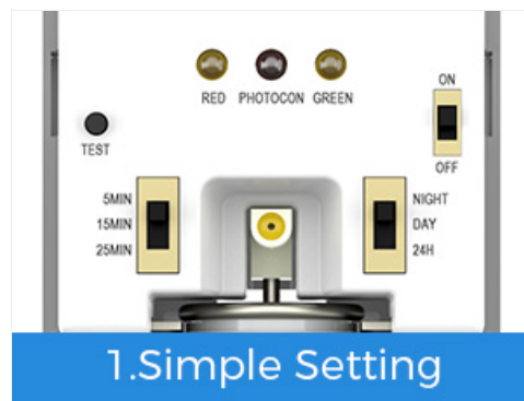
Image 6.1: A detailed view of the dispenser's internal control panel, highlighting the toggle switches for setting spray intervals (5, 15, 25 minutes) and operating modes (NIGHT, DAY, 24H).
