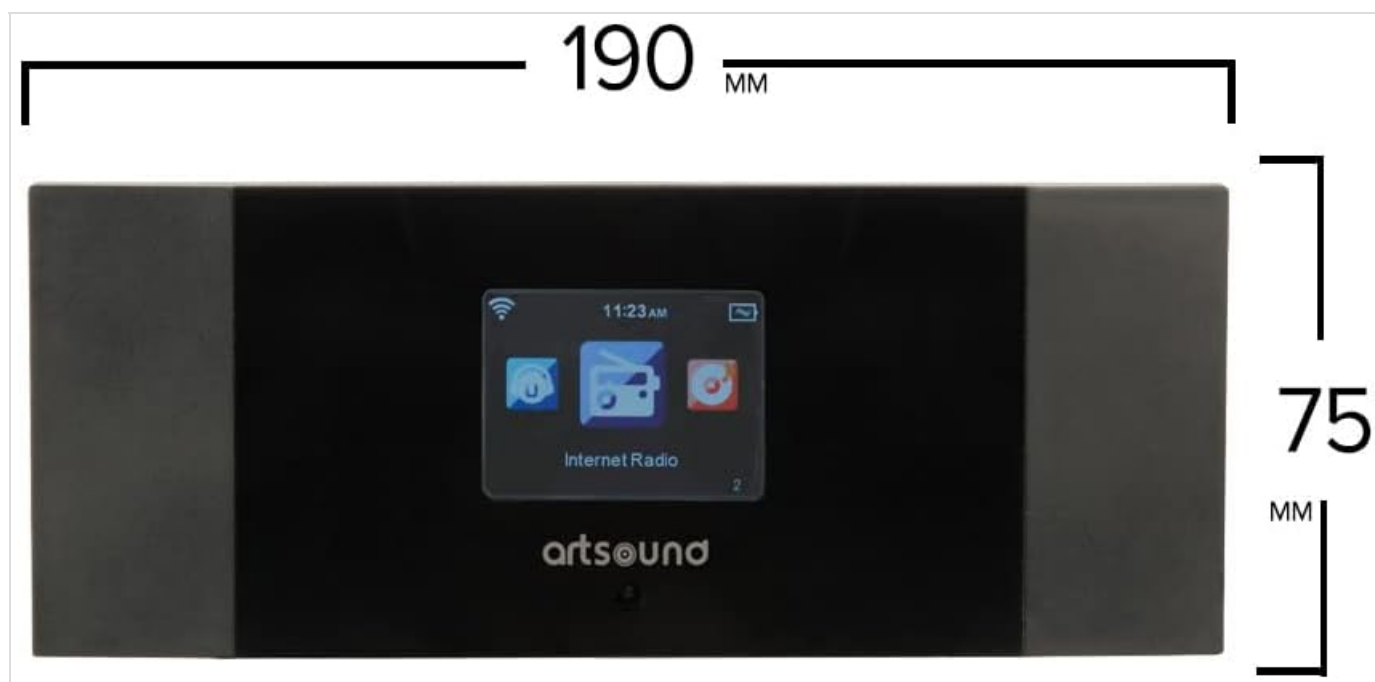
Figure 4.2: ArtSound RI60 Dimensions
