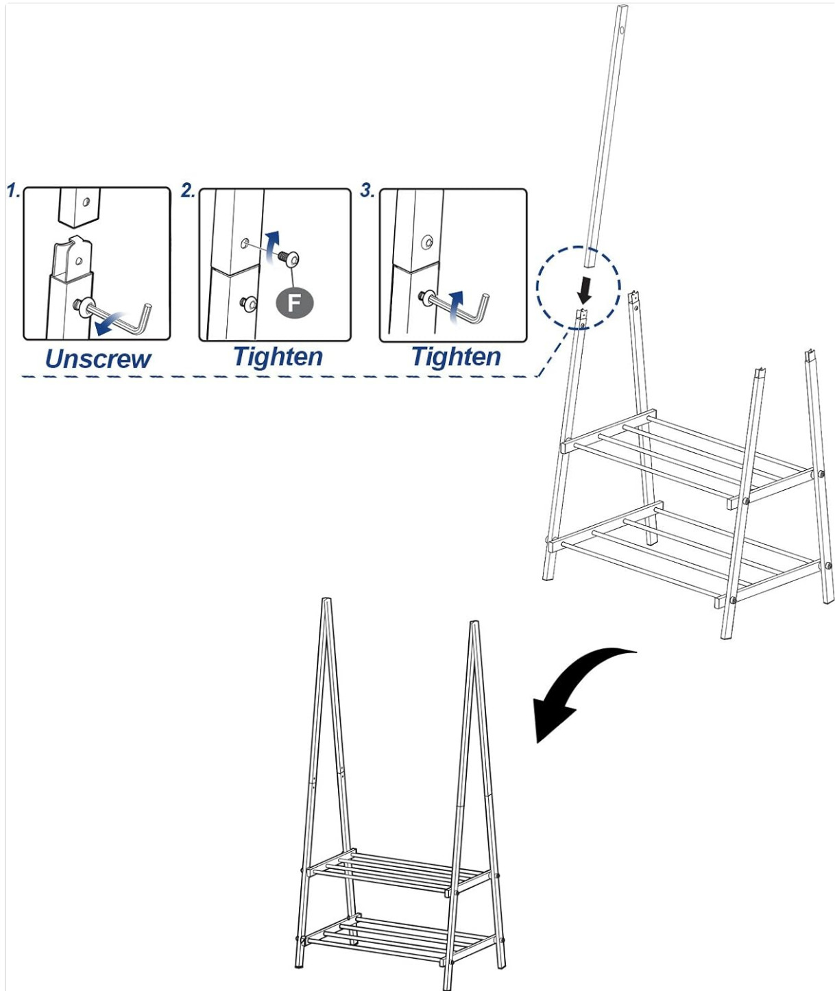
Detailed assembly diagram showing the connection points and parts for the SONGMICS URRCR2B Garment Rack.
