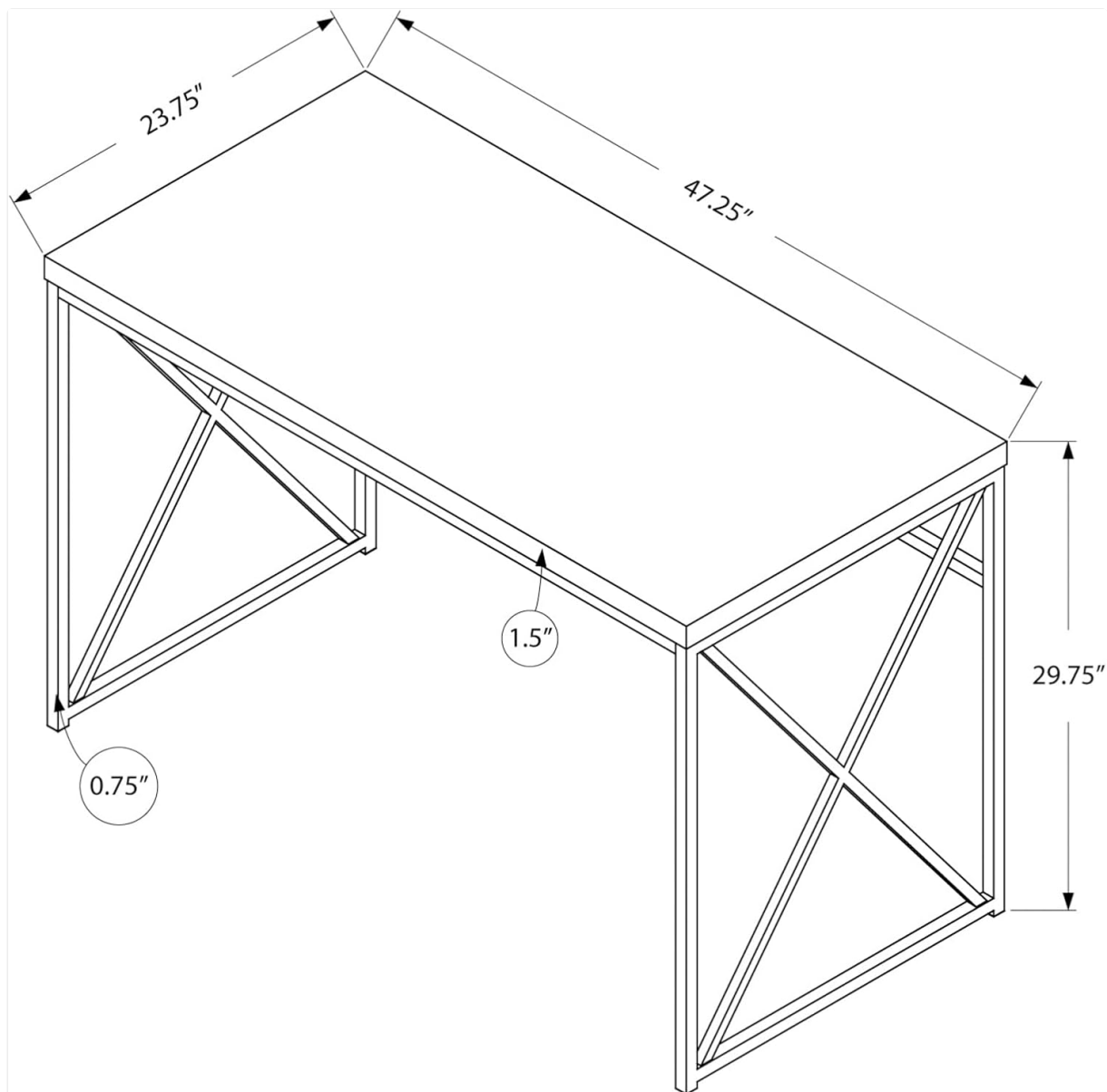
Image: Technical drawing of the desk with key dimensions: 23.75"D x 47.25"W x 29.75"H.
