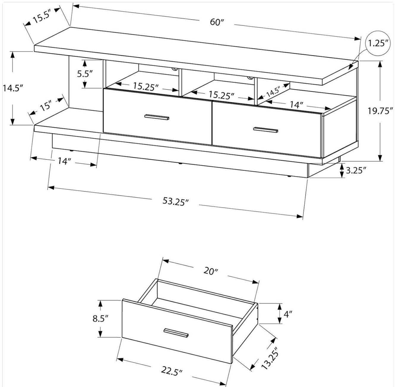
Image 2: Dimensional diagram of the TV Stand, illustrating overall and internal measurements.
