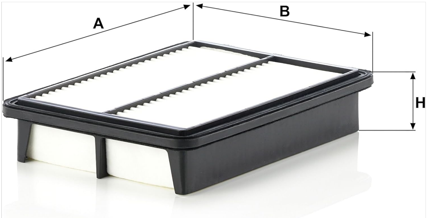
Image 2: Diagram illustrating the dimensions of the MANN-FILTER C 26 032. Labels A, B, and H indicate the length, width, and height respectively, providing a visual reference for the filter's physical size.
