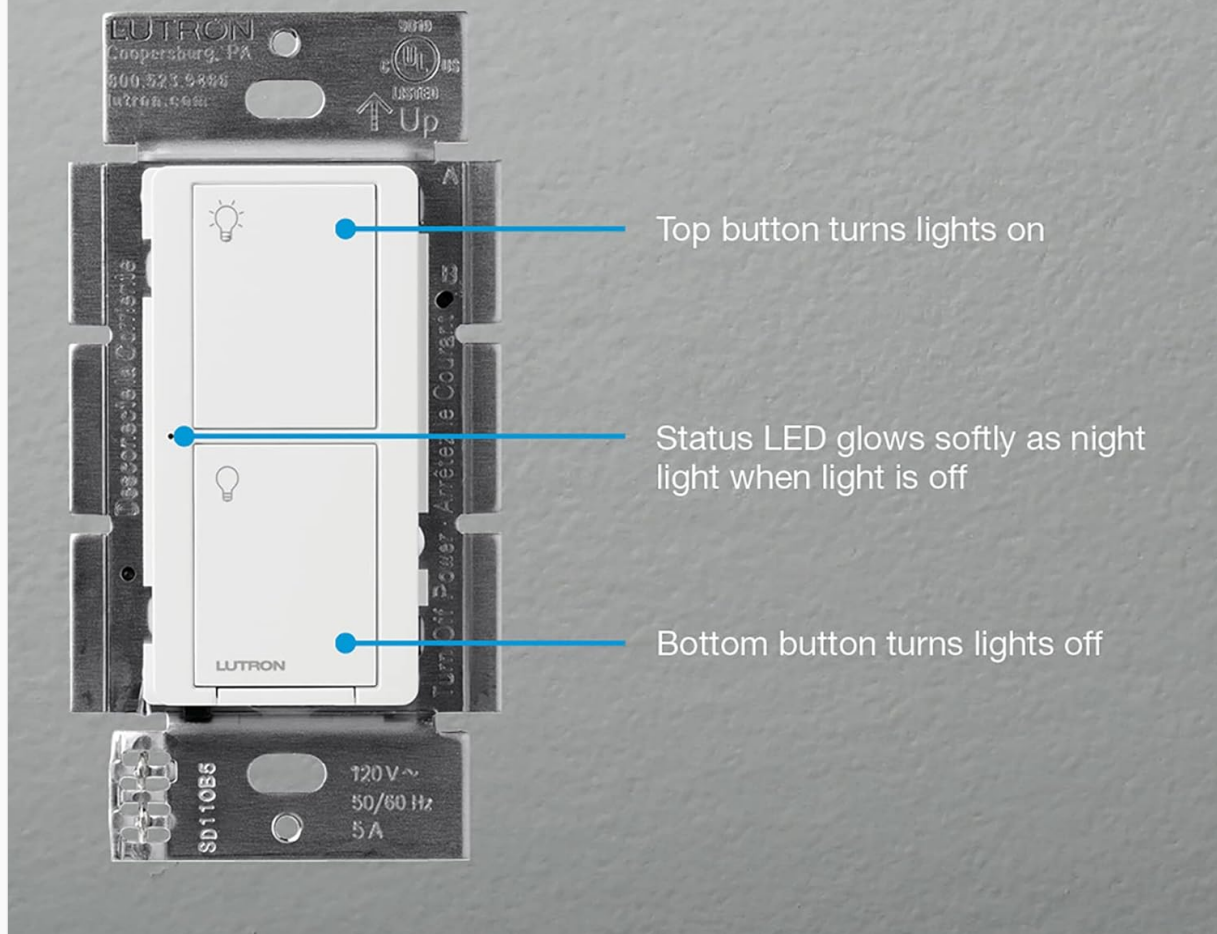
Figure 3: Detailed view of the Caséta Smart Switch face, indicating the top button for turning lights on, the status LED that glows softly when off, and the bottom button for turning lights off.
