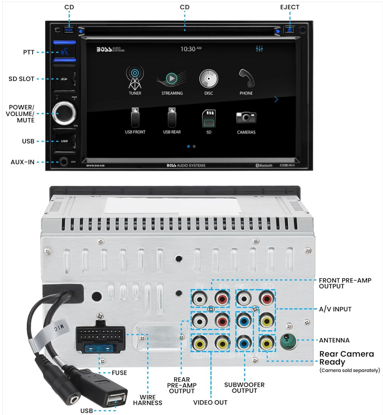
Image 3.2: Front panel controls and rear panel connections diagram.
