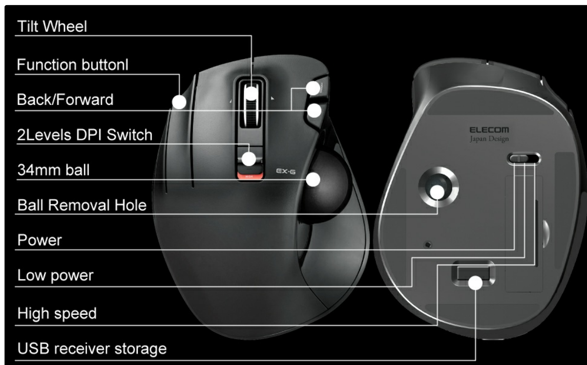
Image: A detailed diagram of the ELECOM EX-G trackball mouse, labeling various components including the 'Ball Removal Hole' on the underside.
